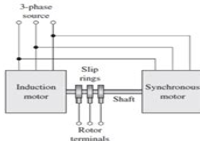
Figure 6.26 Interconnected induction and synchronous machines (Problem 6.8).
